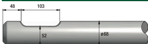
FIGURE 357 SOCOMEK DMS 270
