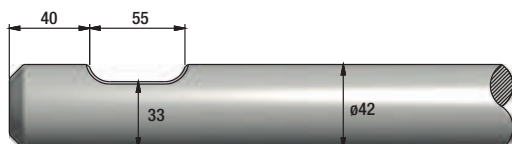
FIGURE 316 RAMMER BR255
