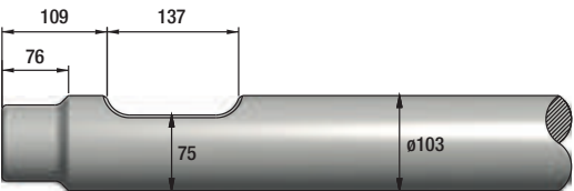
FIGURE 09 ARROWHEAD S130
