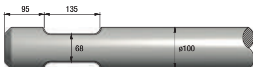
FIGURE 53 EPIROC MB750
