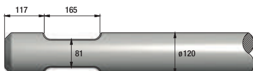
FIGURE 55 EPIROC MB1200
