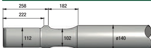
FIGURE 195 MONTABERT V1600
