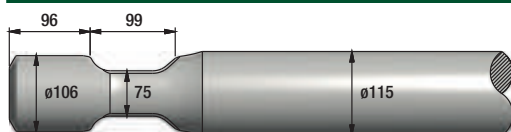
FIGURE 329 RAMMER BR2063
