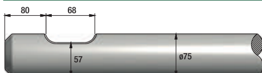
FIGURE 20 CATERPILLAR H75ES
