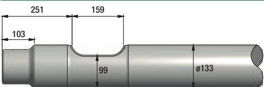
FIGURE 11 ARROWHEAD S230
