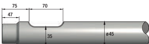
FIGURE 354 SOCOMEK DMS 160
