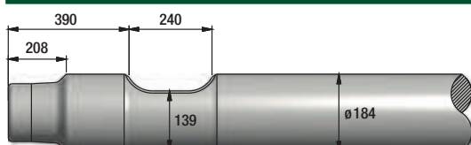
FIGURE 258 NPK E-240A
