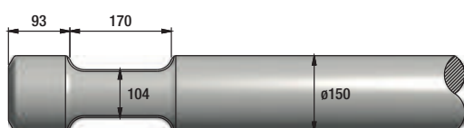
FIGURE 215 MSB SAGA 350
