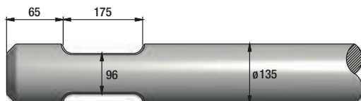
FIGURE 58 EPIROC MB1700
