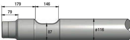
FIGURE 241 NPK E-208A
