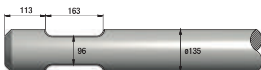
FIGURE 56 EPIROC MB1500
