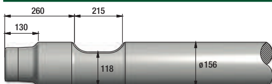
FIGURE 254 NPK E-220
