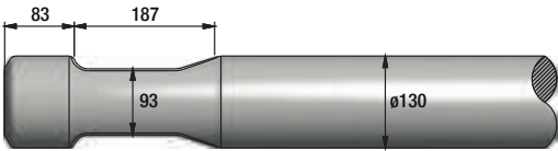
FIGURE 279 PROMOVE XP1500
