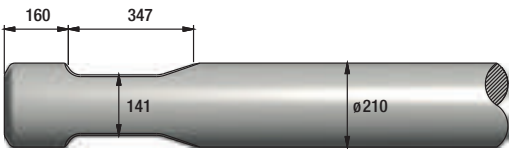
FIGURE 67 EPIROC HB7000
