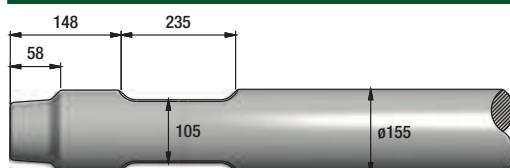
FIGURE 369 SOCOMEK MDO 2050
