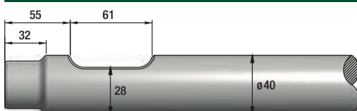
FIGURE 259 NPK H-06X
