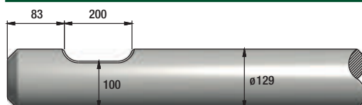
FIGURE 367 SOCOMEK MDO 1450
