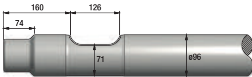
FIGURE 239 NPK E-206
