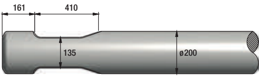
FIGURE 66 EPIROC HB5800
