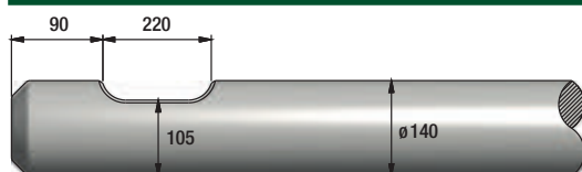
FIGURE 368 SOCOMEK MDO 1950
