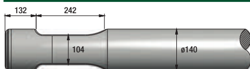
FIGURE 196 MONTABERT V1800
