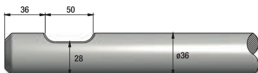
FIGURE 315 RAMMER BR222
