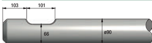
FIGURE 326 RAMMER BR999
