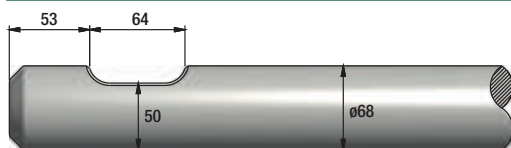
FIGURE 19 CATERPILLAR H65ES
