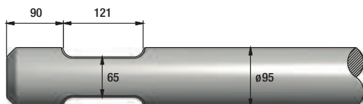
FIGURE 45 EPIROC SB552
