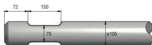
FIGURE 46 EPIROC HBC1100 / 1700
