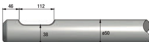
FIGURE 318 RAMMER BR333
