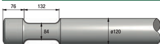
FIGURE 212 MSB SAGA 180
