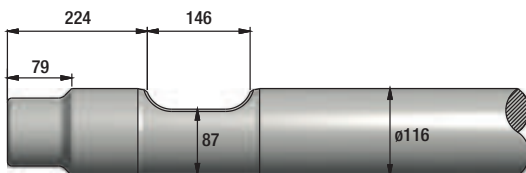
FIGURE 242 NPK GH7
