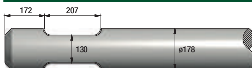
FIGURE 371 SOCOMEK MDO 4000
