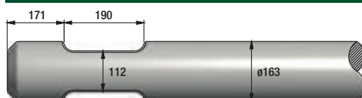
FIGURE 370 SOCOMEK MDO 3000 / 3200
