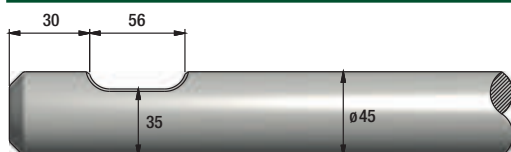
FIGURE 352 SOCOMEK DMS 50
