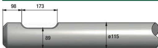
FIGURE 365 SOCOMEK MDO 750
