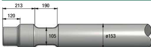
FIGURE 215 MSB SAGA 350
