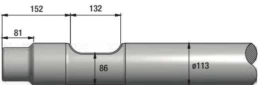
FIGURE 10 ARROWHEAD S180
