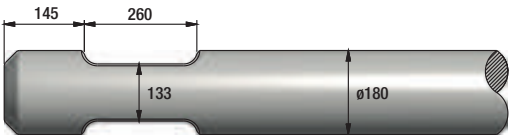
FIGURE 281 PROMOVE XP4500
