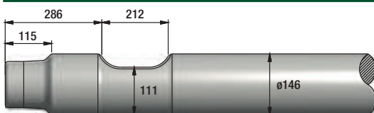
FIGURE 245 NPK GH12
