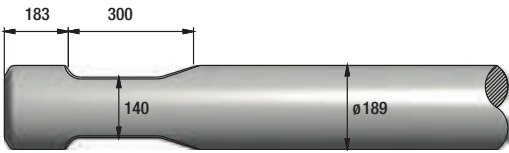
FIGURE 65 EPIROC HB4700
