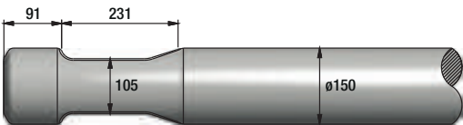
FIGURE 280 PROMOVE XP2400
