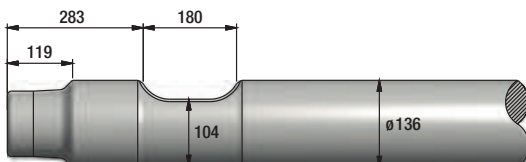
FIGURE 244 NPK GH10
