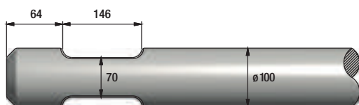
FIGURE 46 EPIROC HBC1100 / 1700
