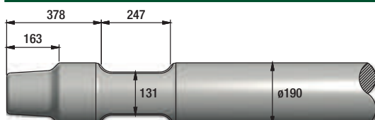
FIGURE 257 NPK E-235
