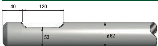
FIGURE 355 SOCOMEK DMS 210
